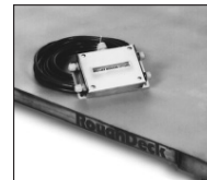
Remote EL604STA stainless steel NEMA 4X junction box with 20 ft of hostile environment load cell cable.
